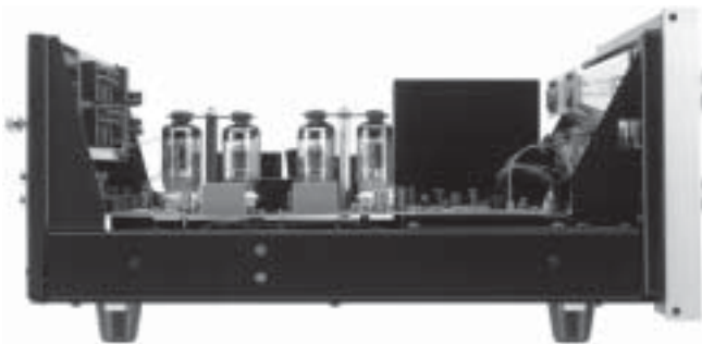
Side Inside View of the C2200
