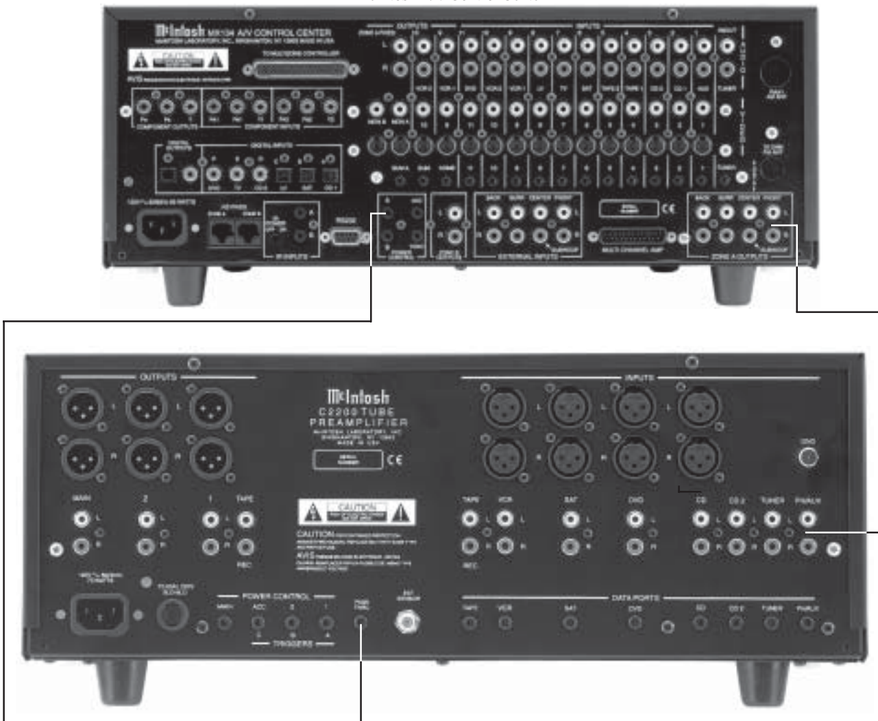
McIntosh A/V Control Center
