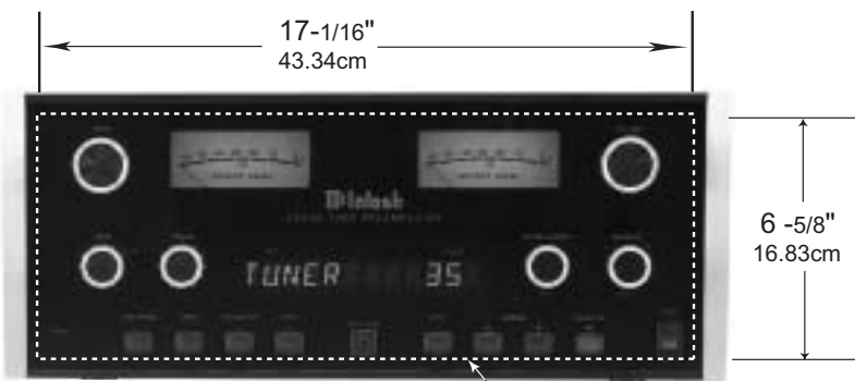
C2200 Front Panel Custom Cabinet Cutout
